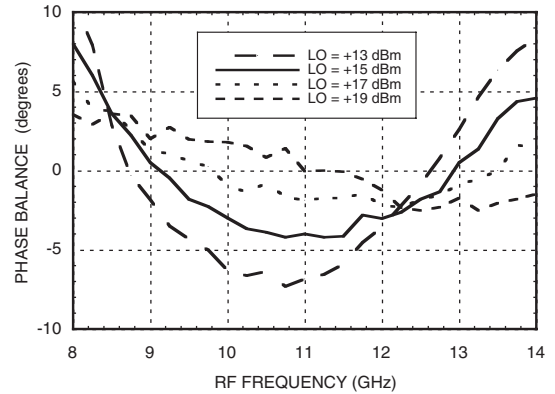
Phase Balance vs. LO Drive
