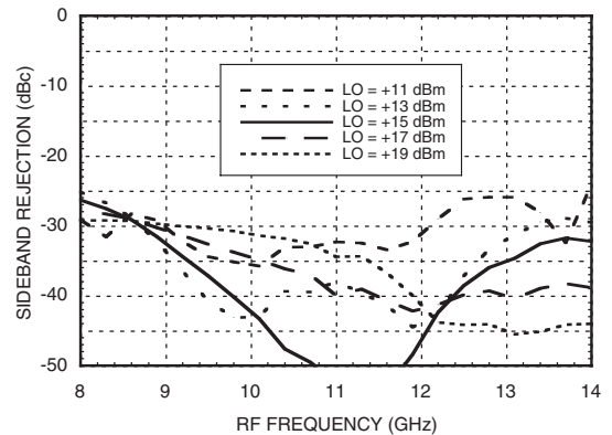
Upconverter Performance Sideband Rejection vs. LO Drive
